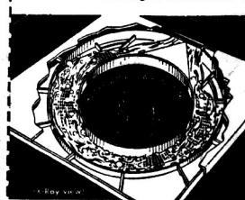
X-Ray view of lid showing lint filtering action during wash and rinse cycles.
