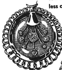
Locket & chain
